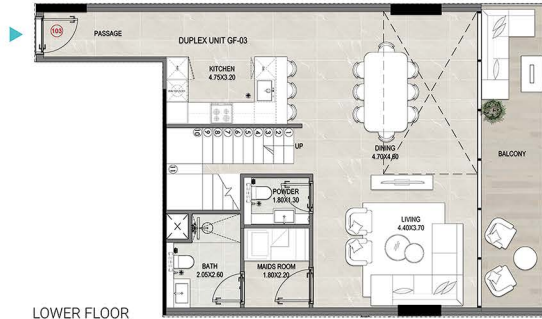
LOWER FLOOR
