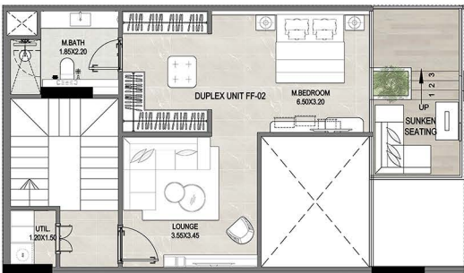
UPPER FLOOR
