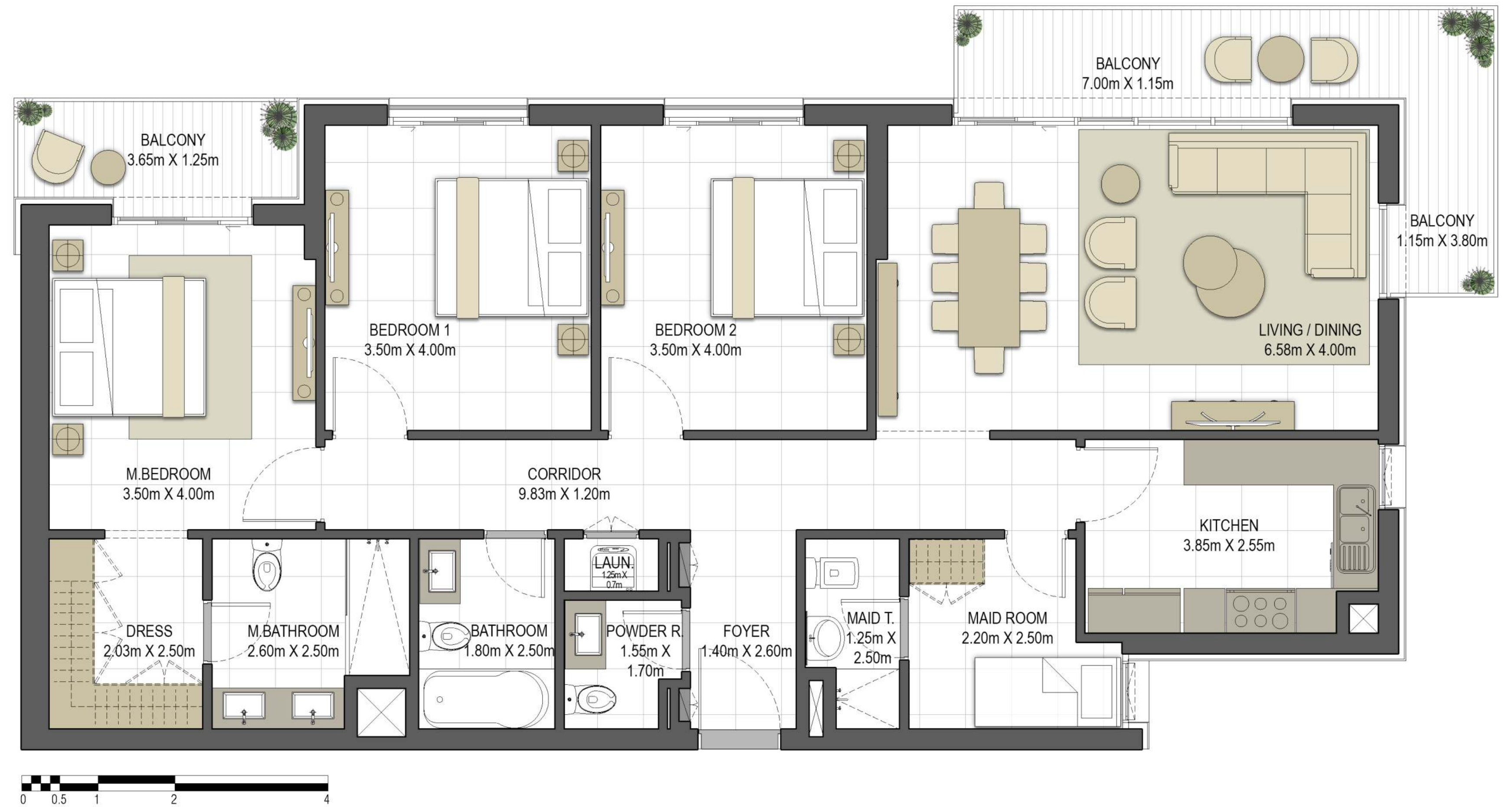
LEVEL 01
