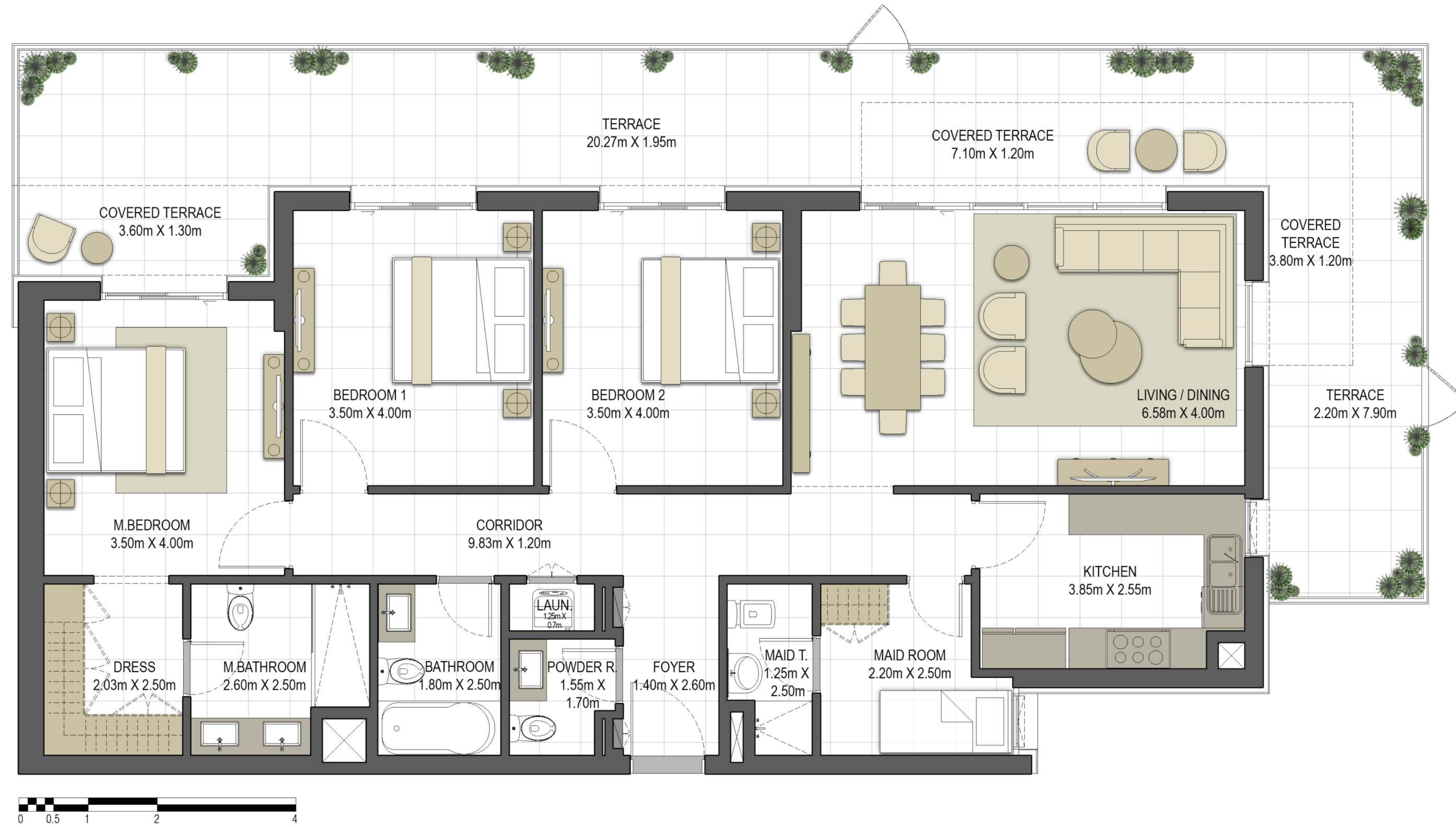
LEVEL 01
