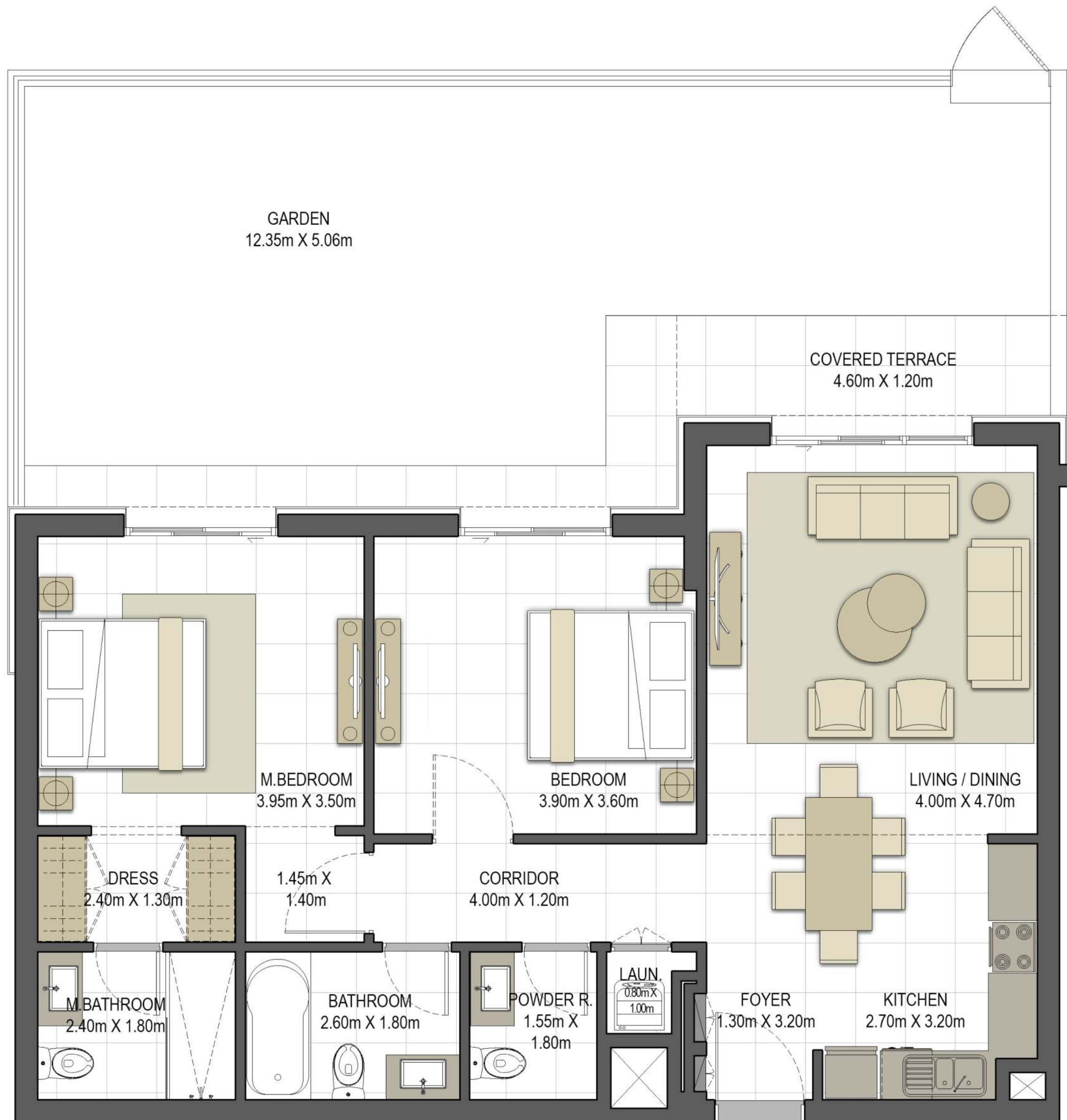
LEVEL 01
