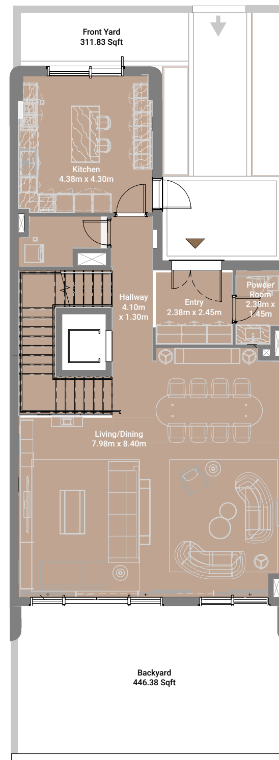
Level 02
