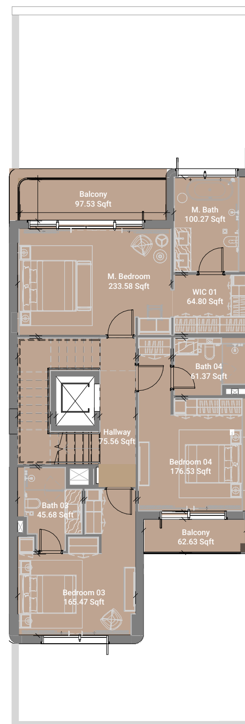
Level 03
