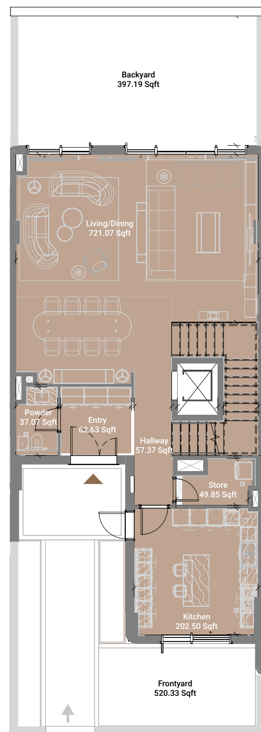
Level 02
