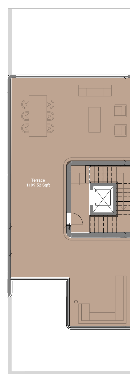
Roof Level
