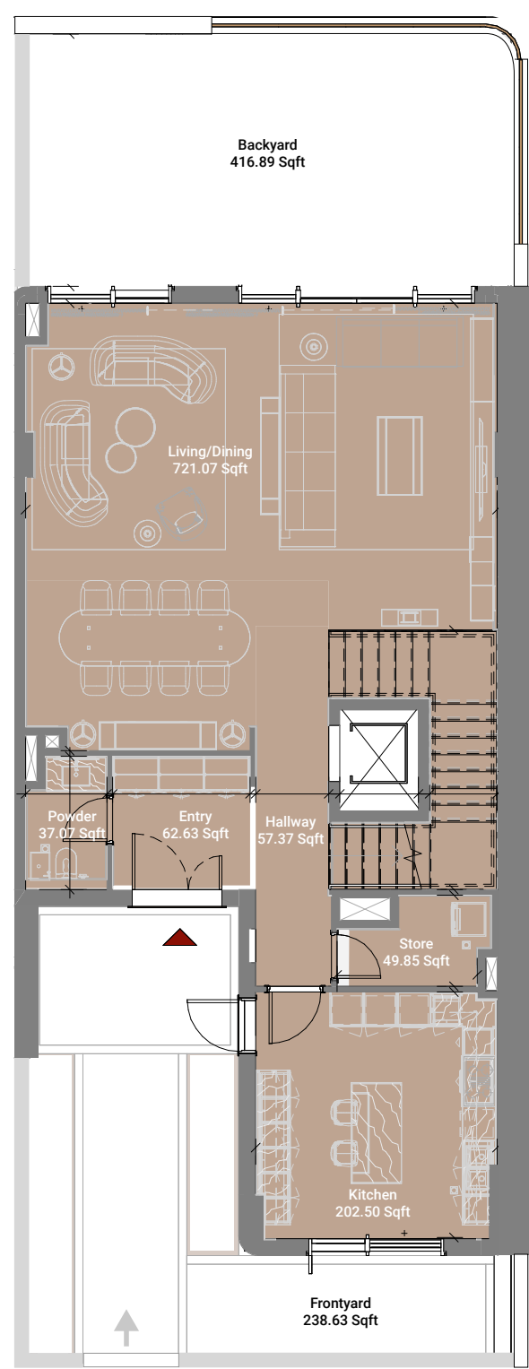
Level 02
