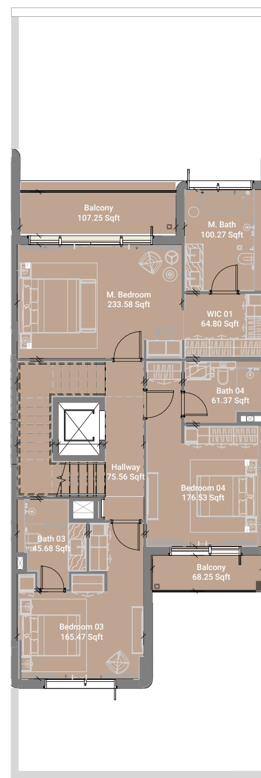
Level 03
