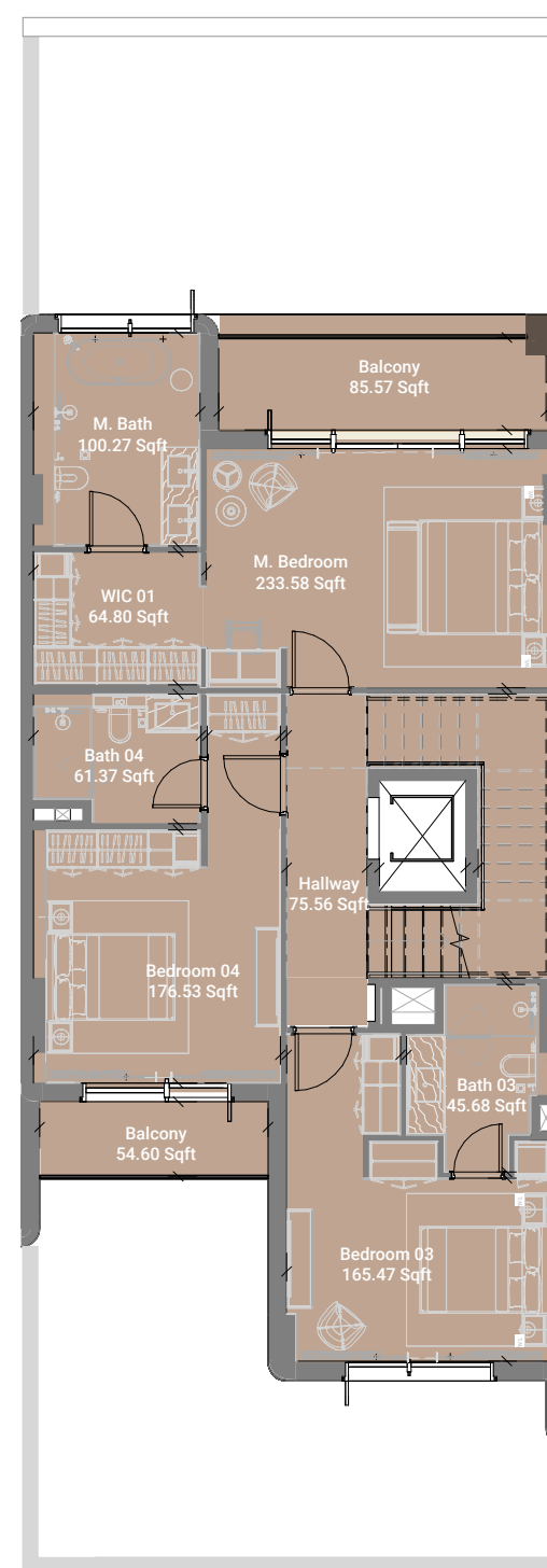
Level 03
