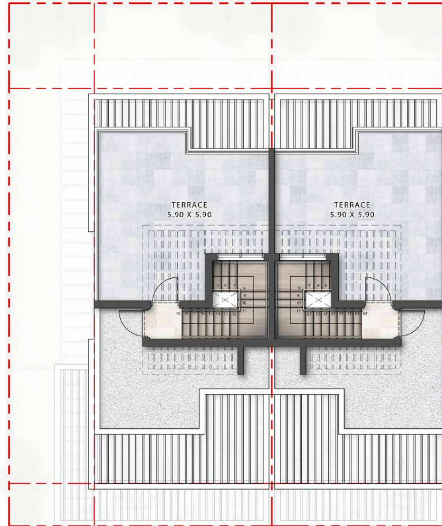
ROOF FLOOR
