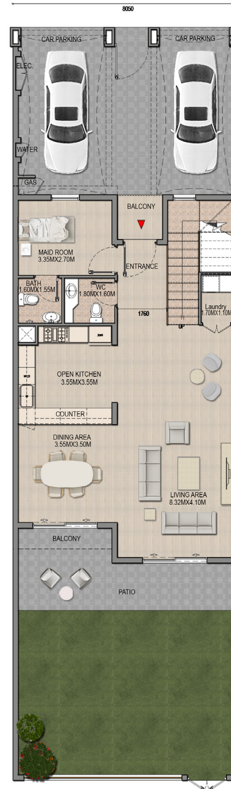
Ground Floor
