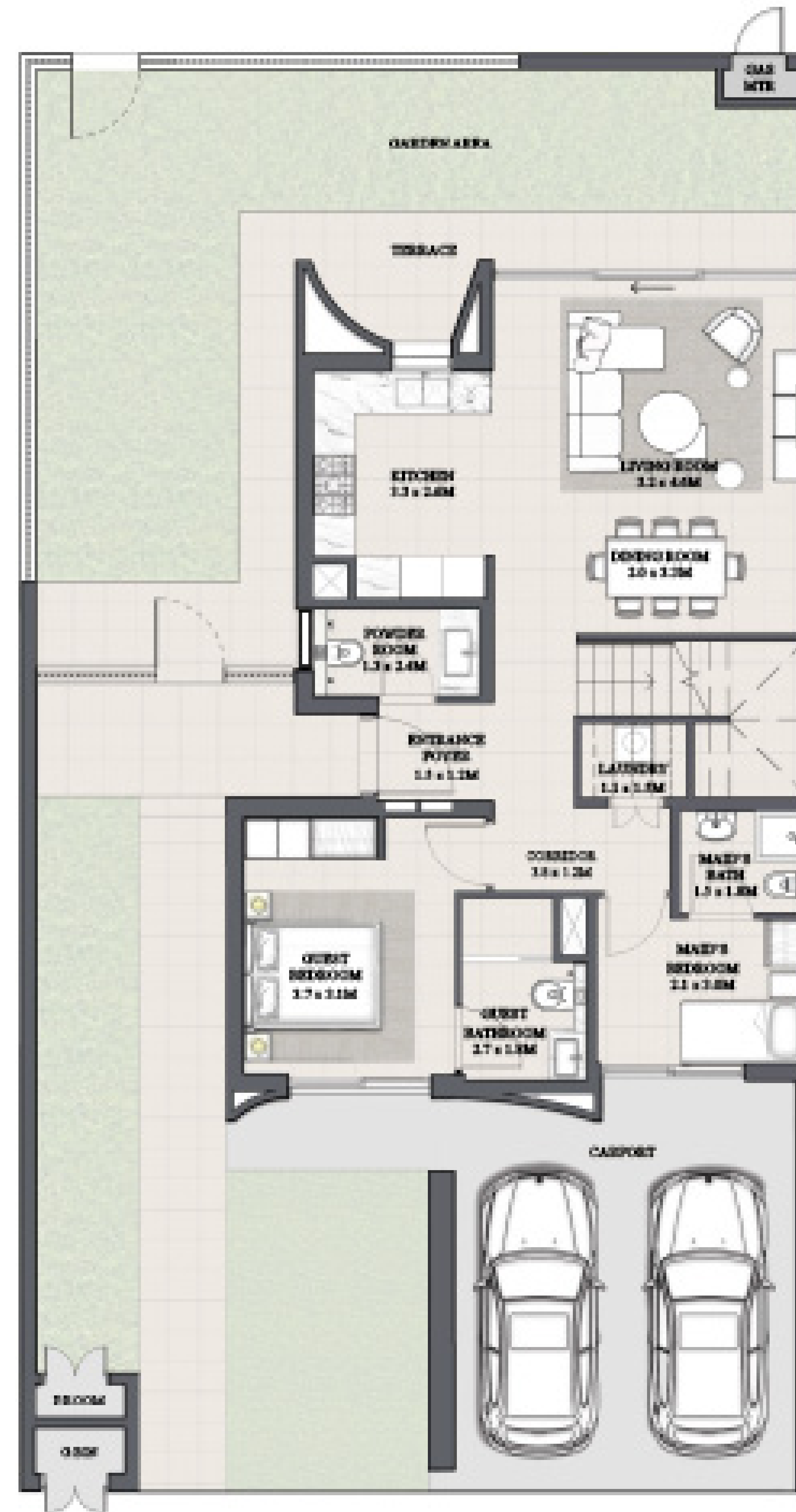
GROUND FLOOR
