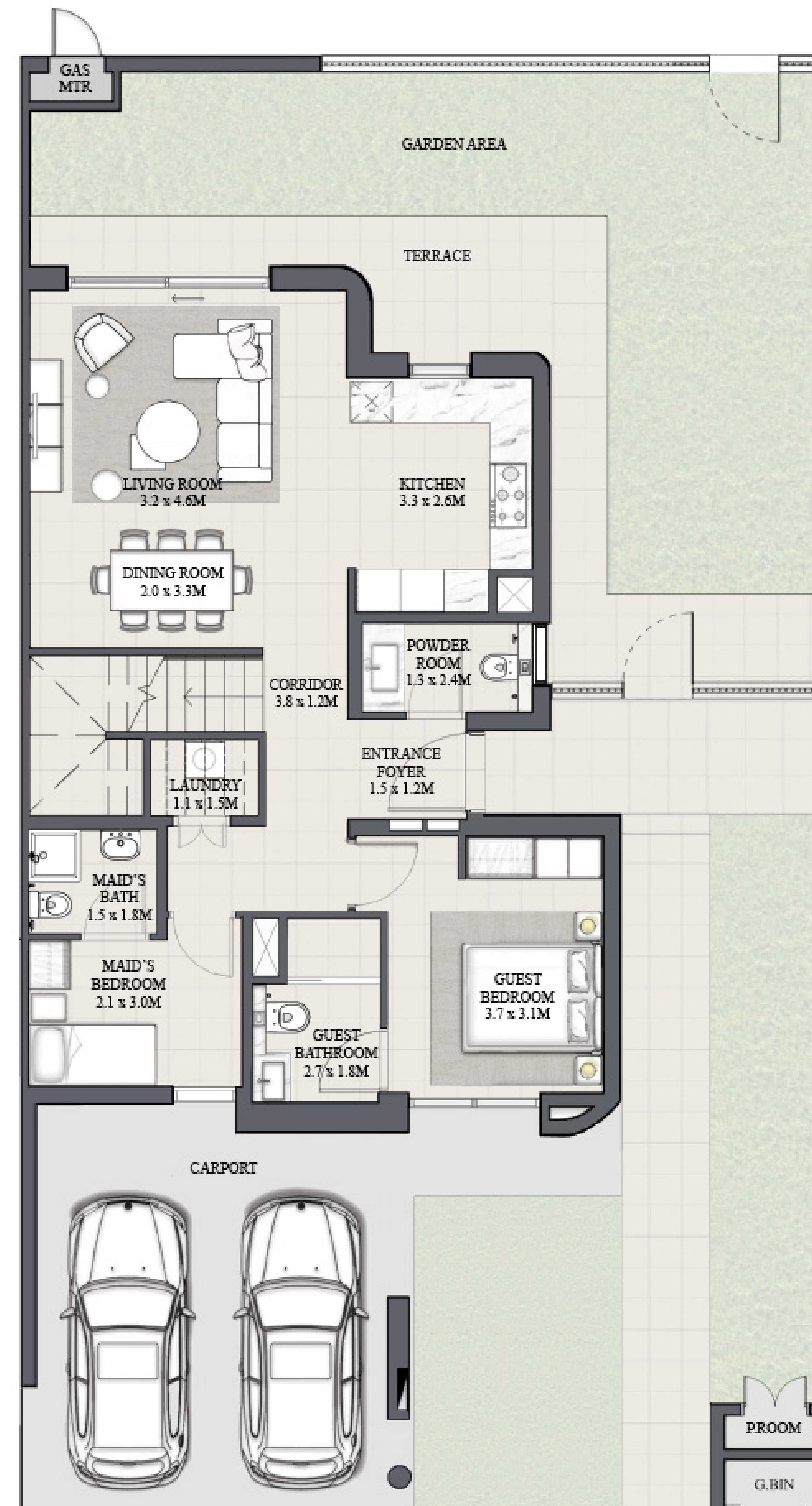
GROUND FLOOR
