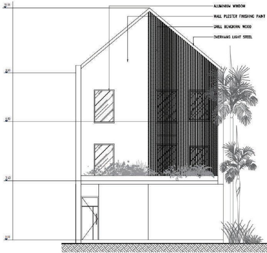
FRONT ELEVATION
