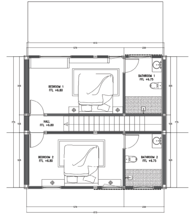
2 ND FLOOR
