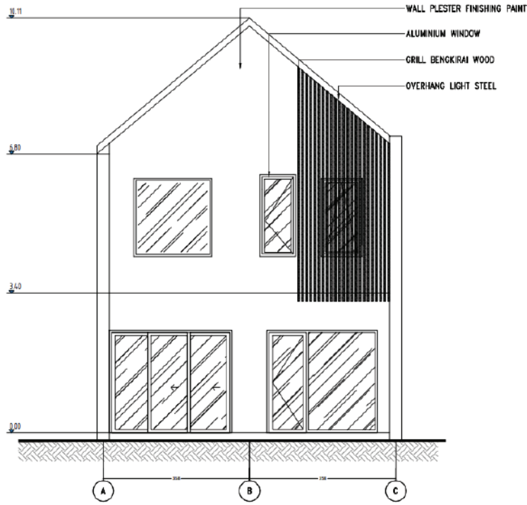
REAR ELEVATION
