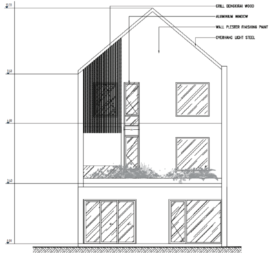
REAR ELEVATION
