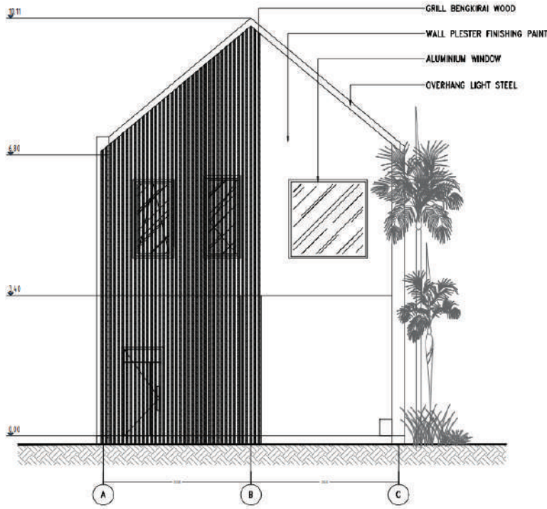
FRONT ELEVATION
