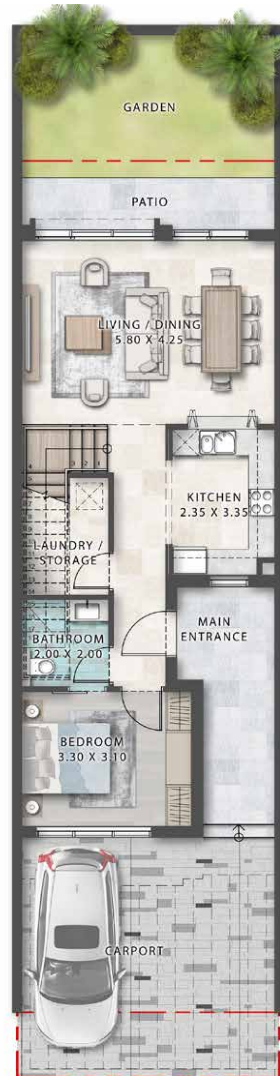
GROUND FLOOR
