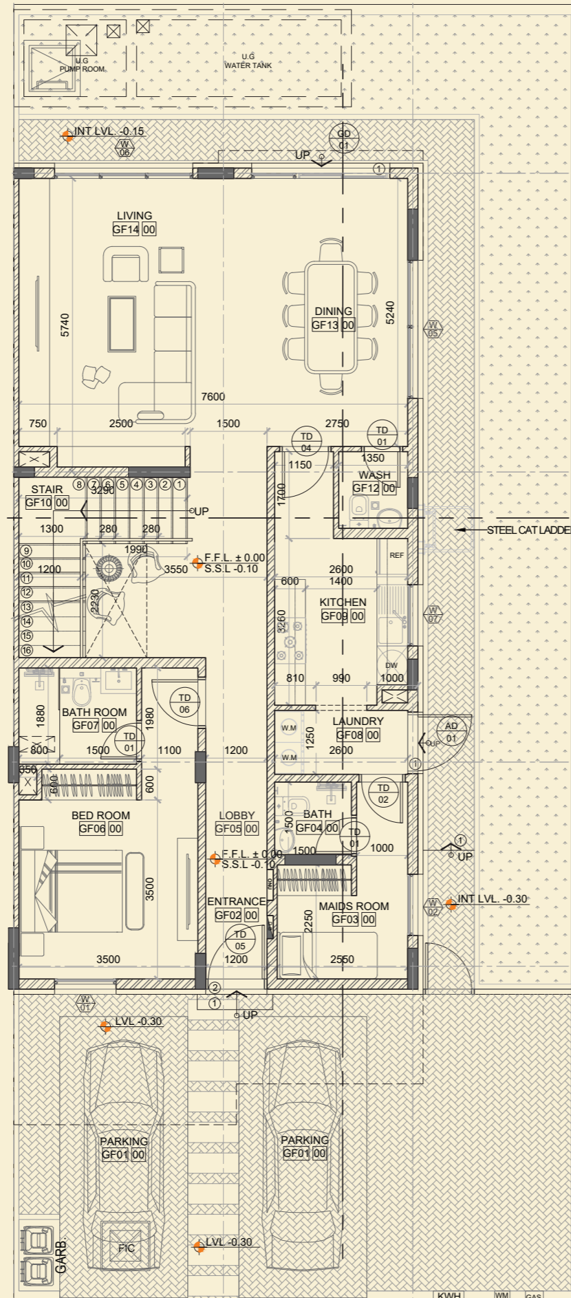
GROUND FLOOR
