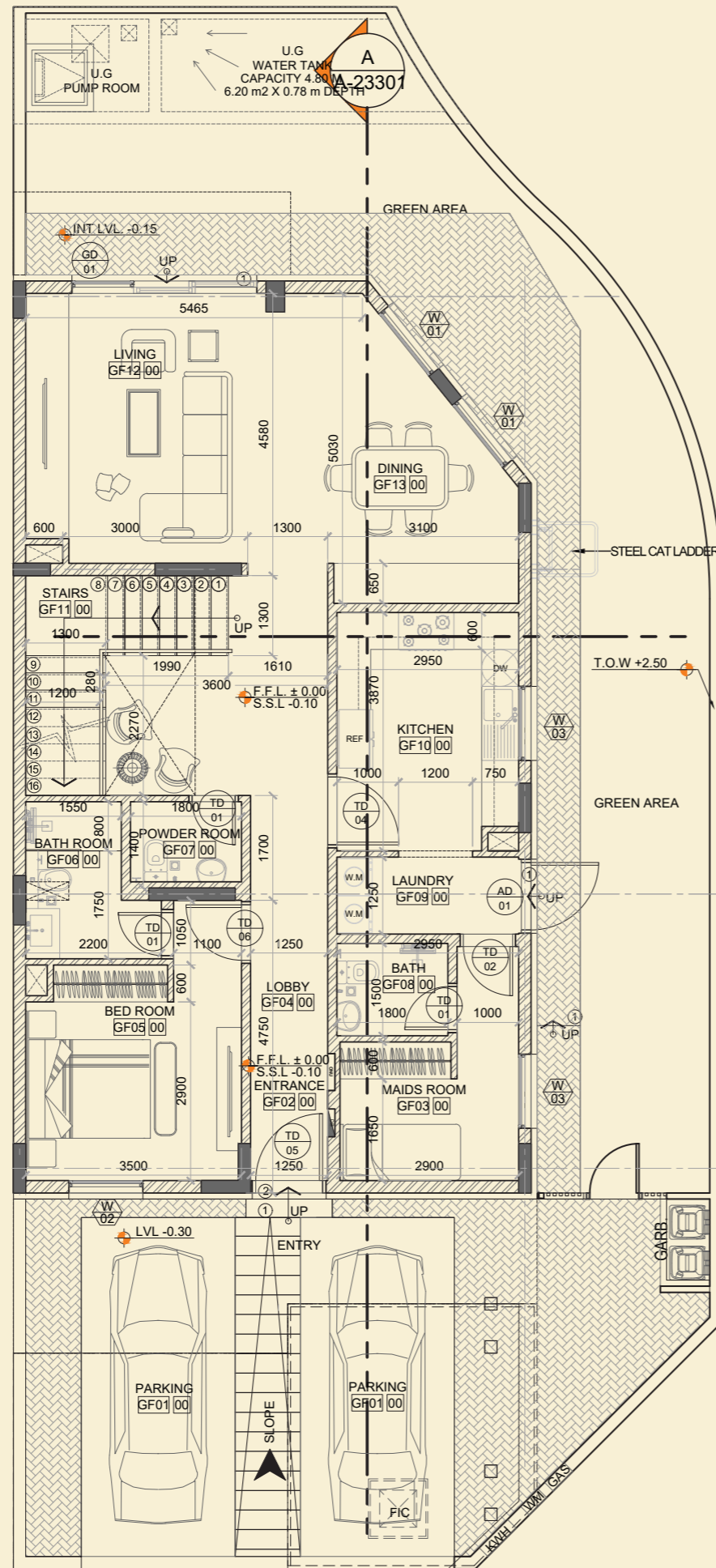
GROUND FLOOR
