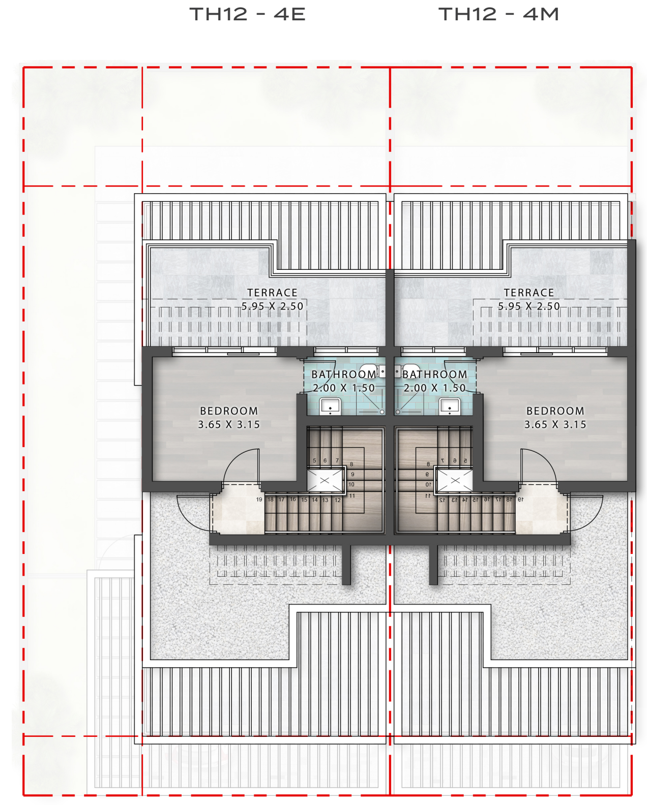
ROOF FLOOR
