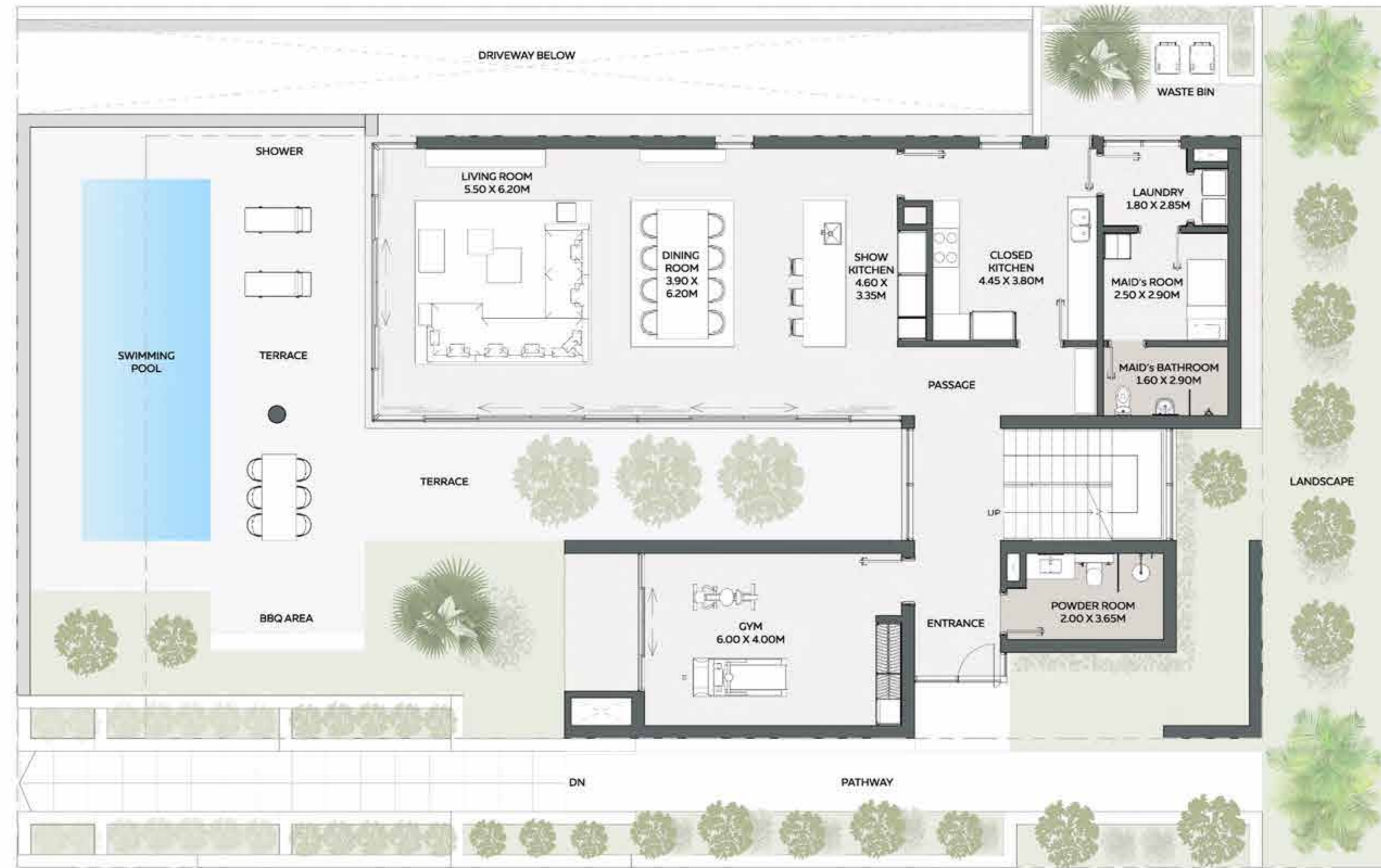
GROUND FLOOR
