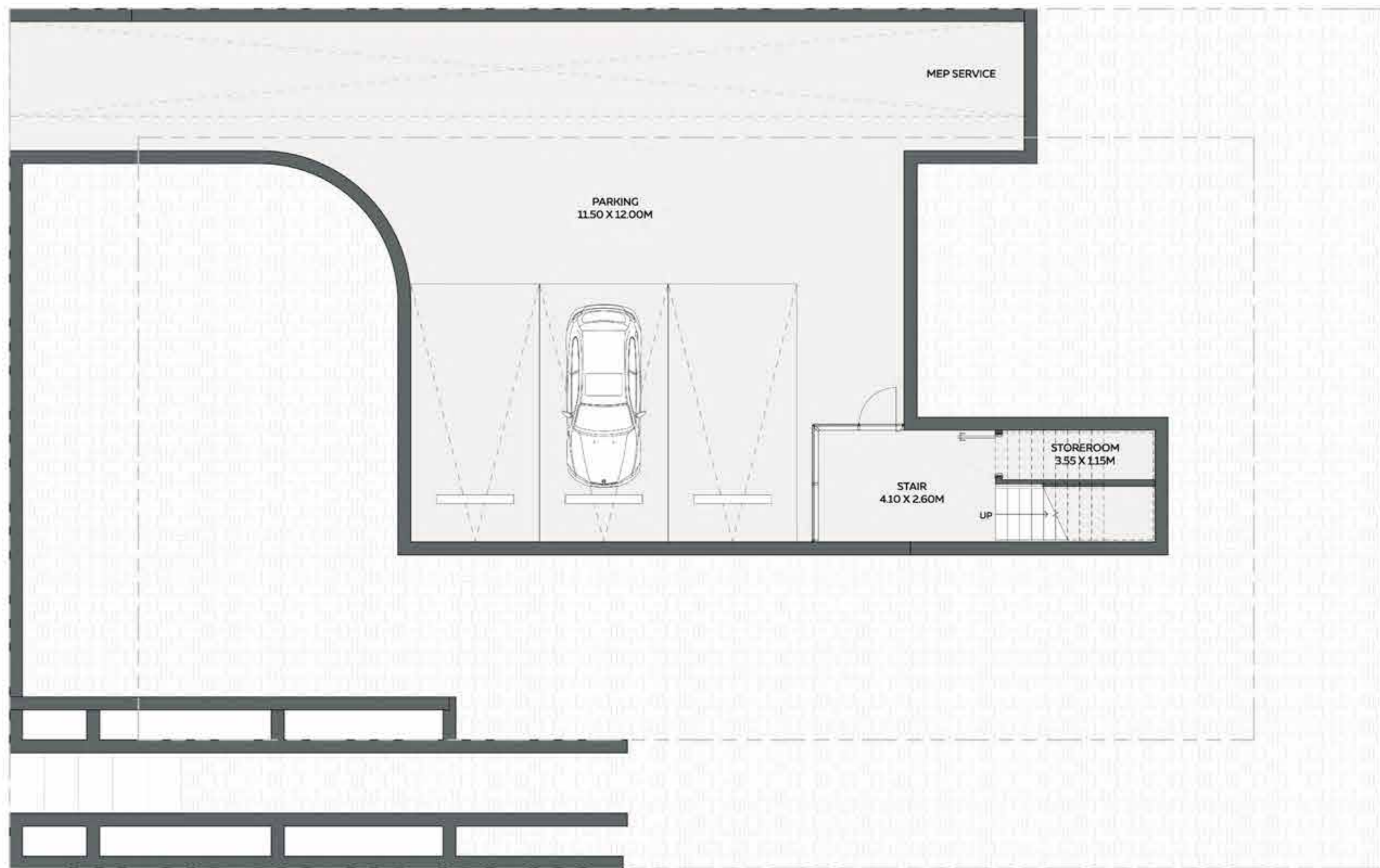
ROOF FLOOR
