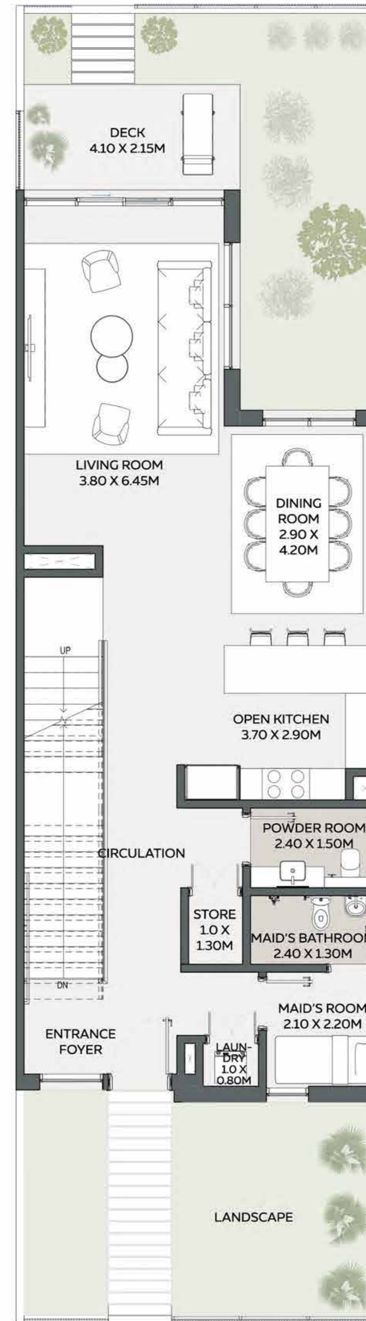
GROUND FLOOR
