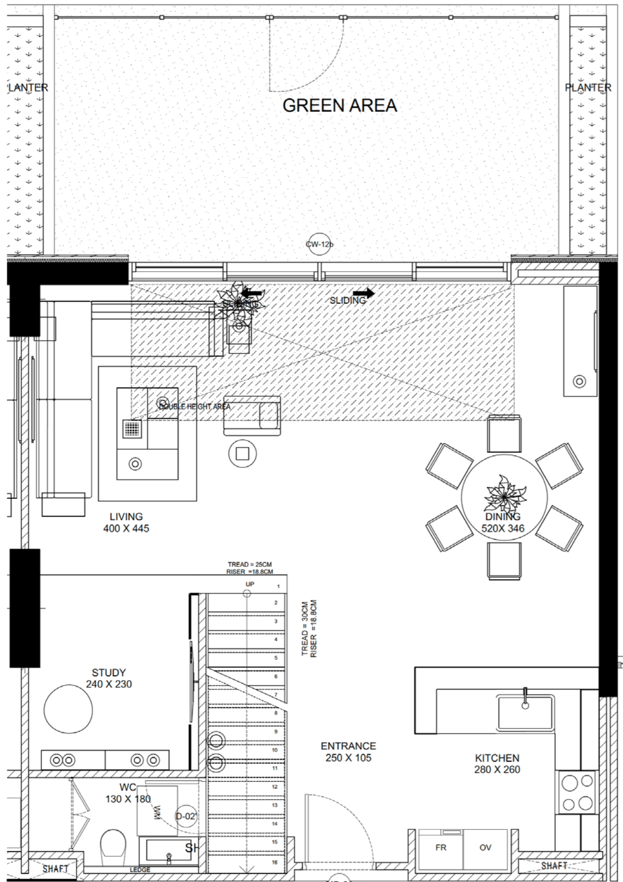
Lower Floor
