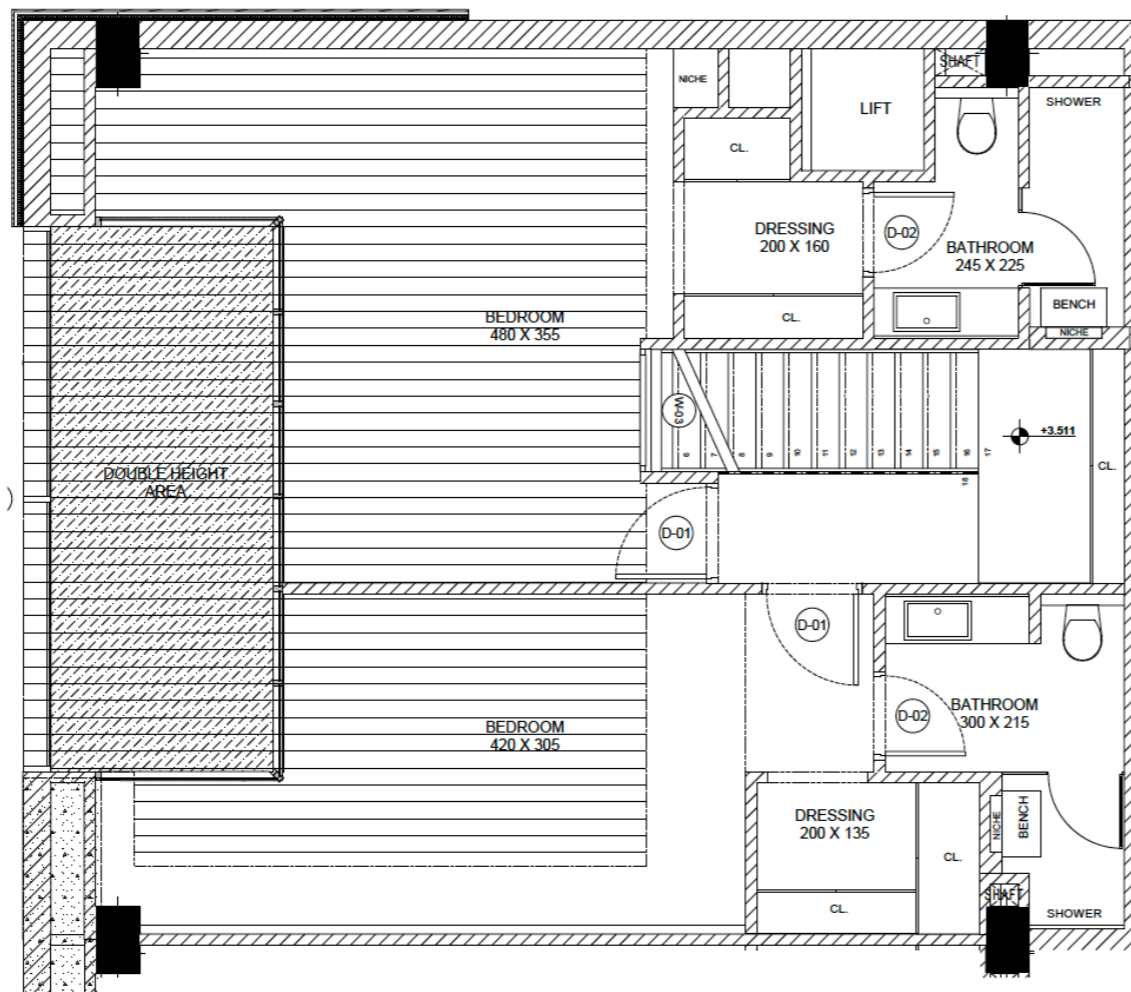
Upper Floor
