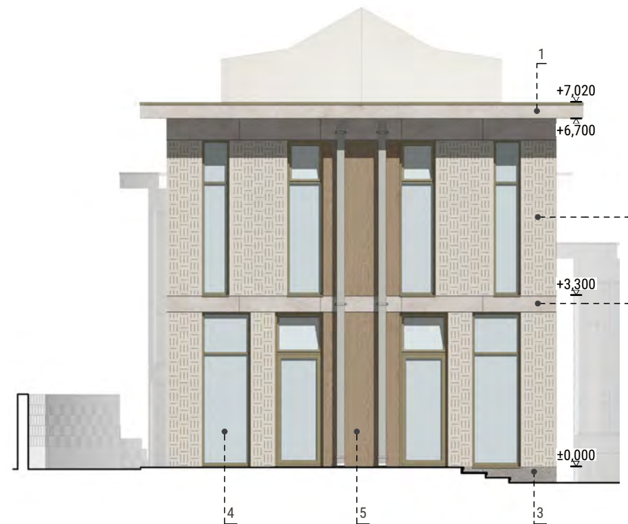
ELEVATION 2-2
