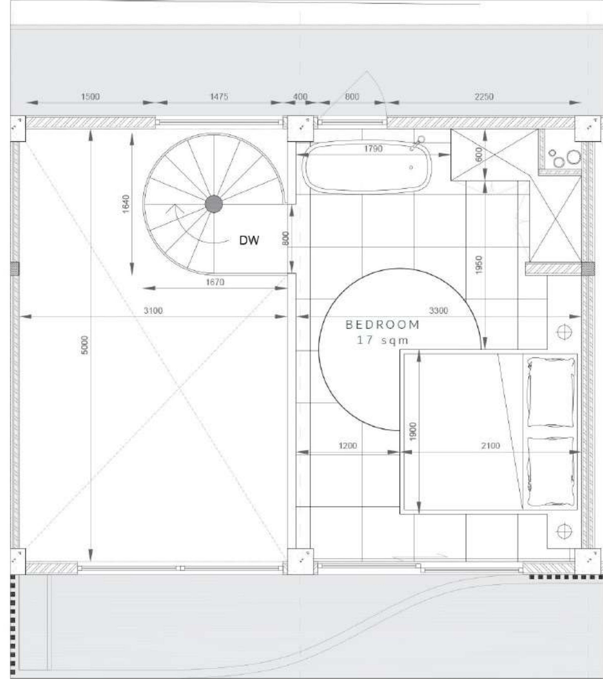
MEZZANINE PLAN
