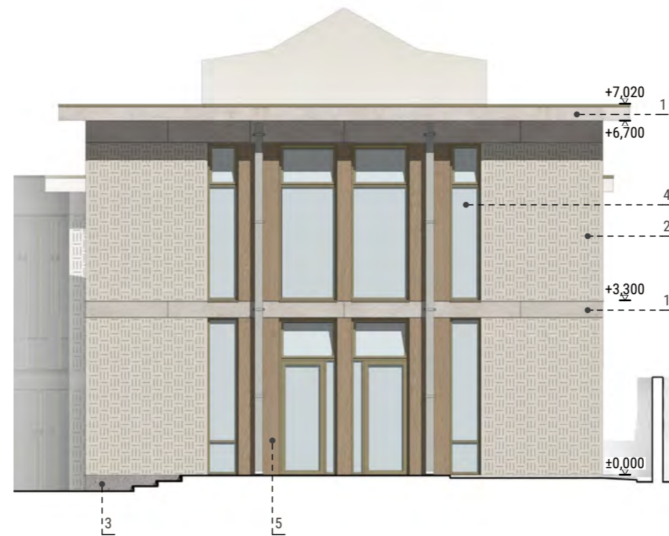
ELEVATION 2-2
