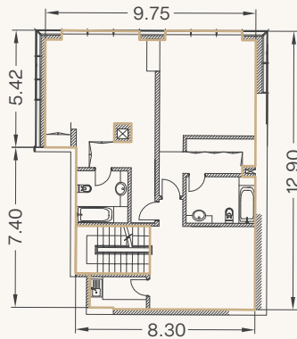
Lower Ground
