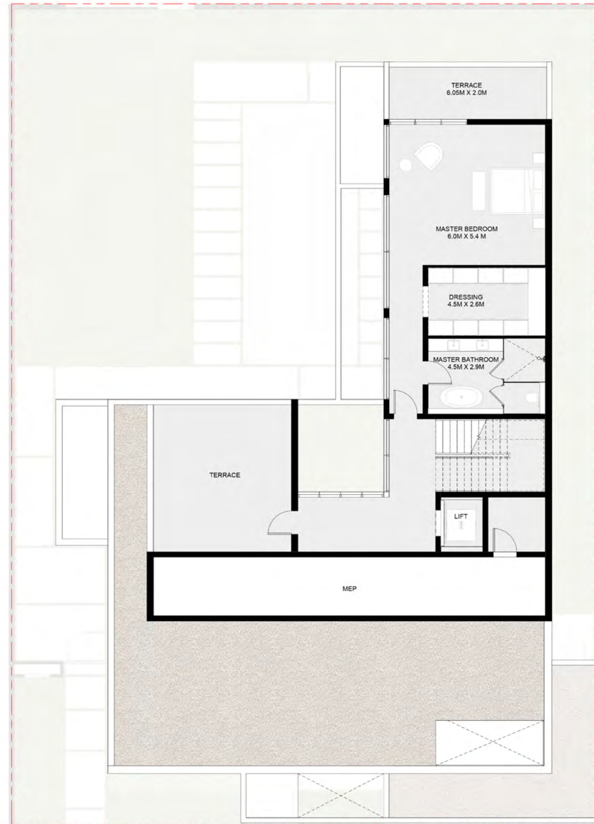
Second Floor
