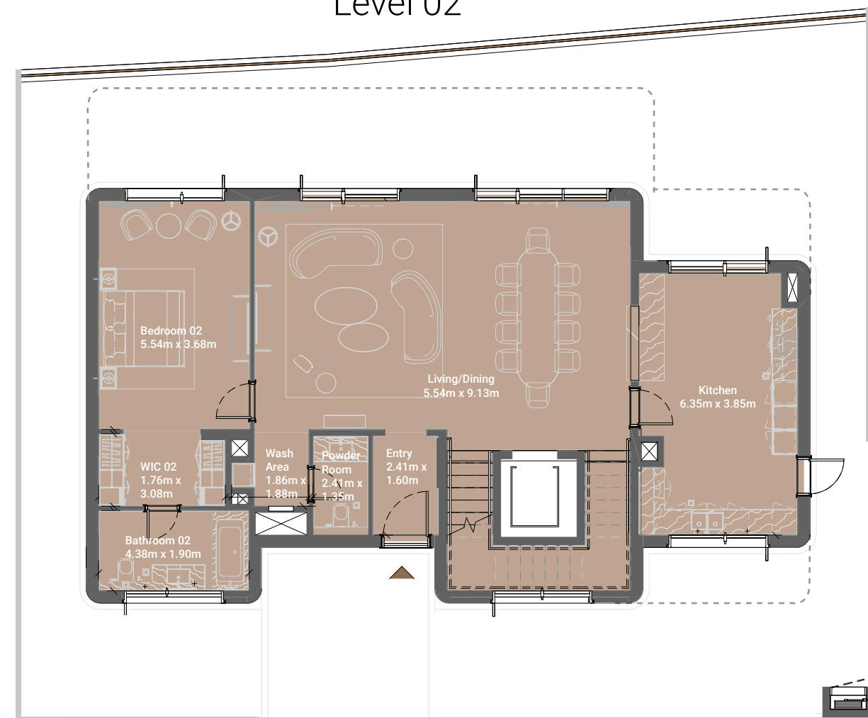
Level 02
