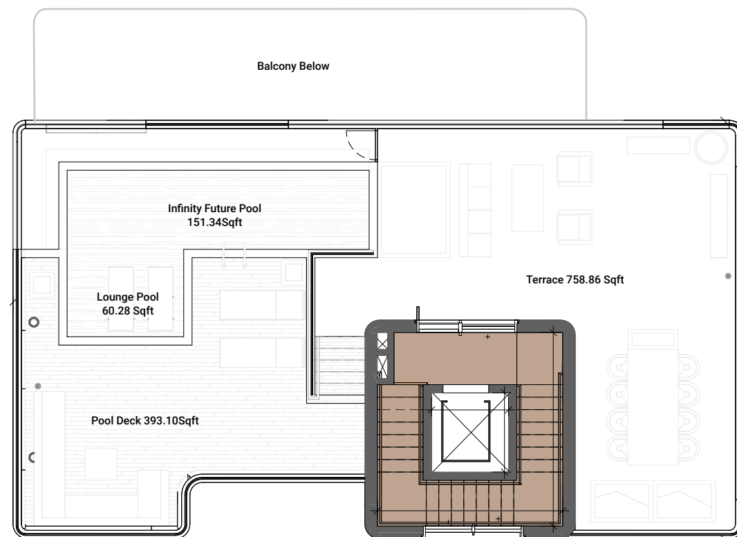
Roof Level
