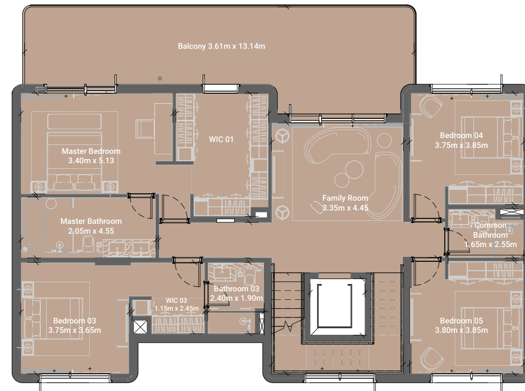
Level 03
