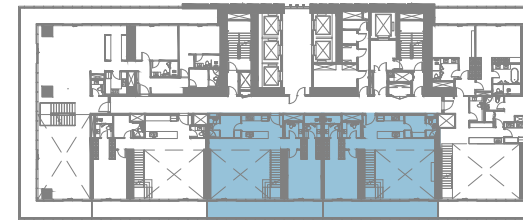
11TH FLOOR
