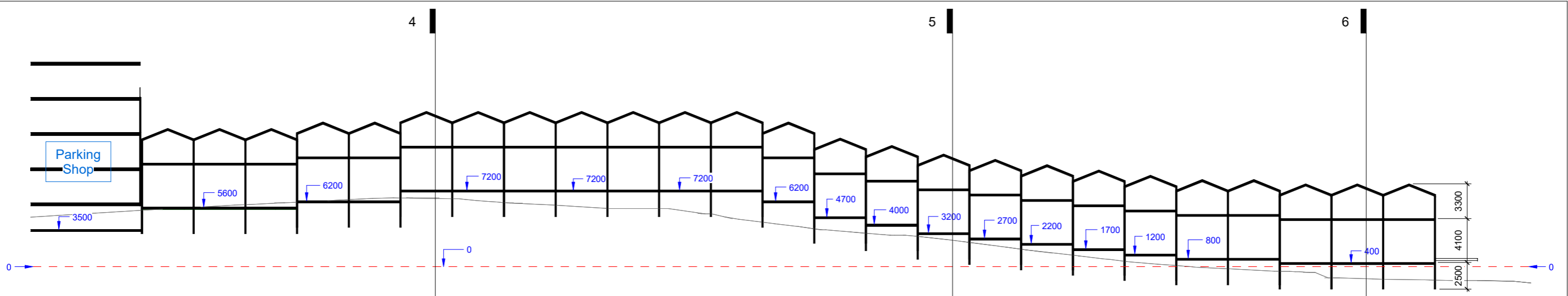
Section 1-1
