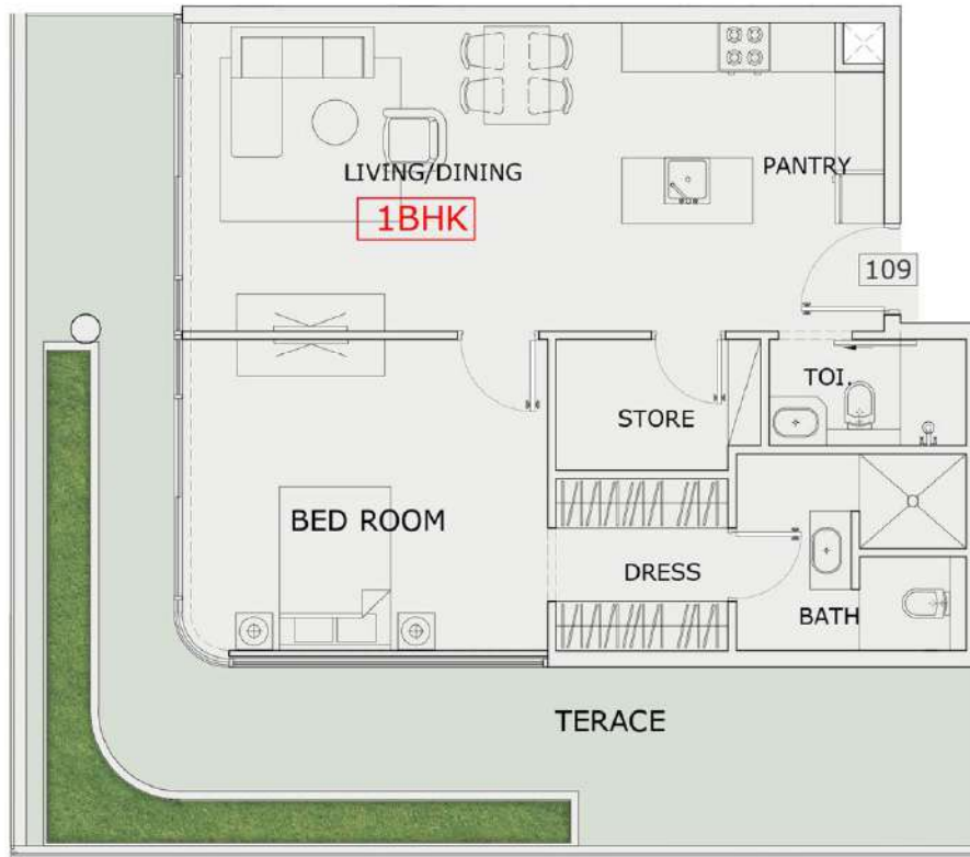
UNIT - 109
